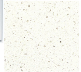
Quartz
