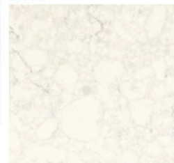
Quartz
