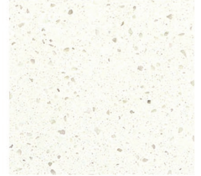
Quartz
